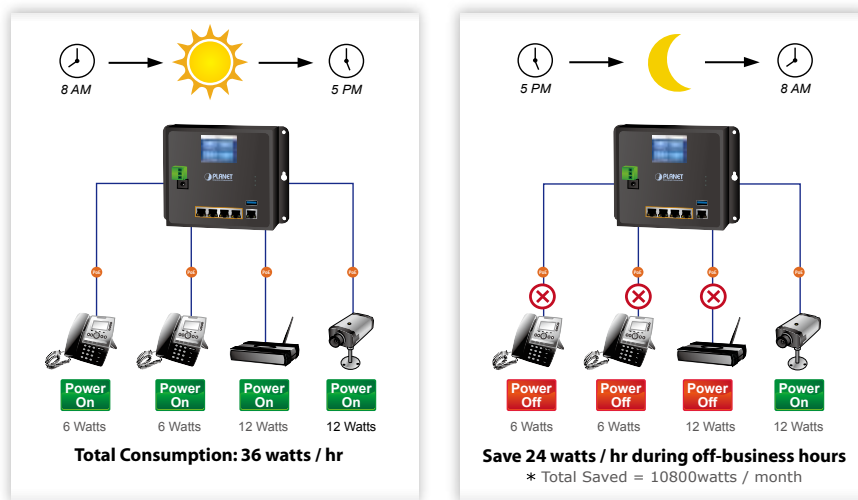
1000BASE-TX UTP with PoE
