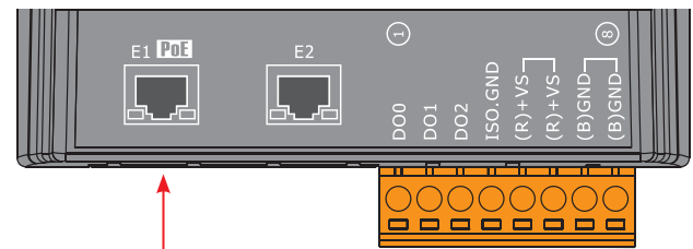
PET-7219: PoE
