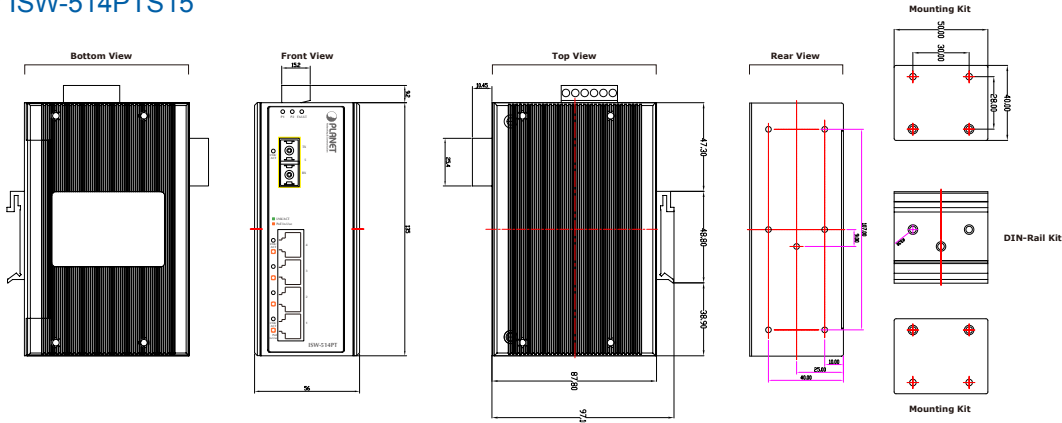
ISW-514PT / ISW-514PTS15
