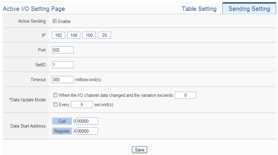
Figure 8-38 : “Active Sending of I/O Data Table” Setting page (2)
