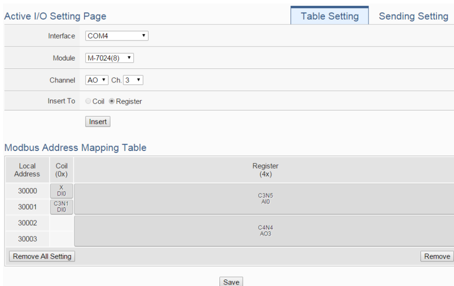
Figure 8-36 : I/O Data Table Setting page (2)
